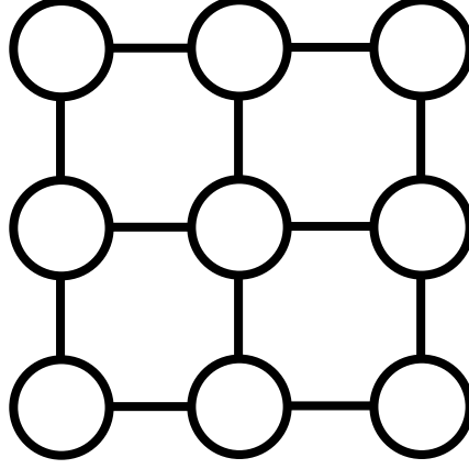
Figure 2.1: The Ising model is a probabilistic model used in statistical physics. The nodes in this probabilistic graphical model represent random variables, and the edges in the graph represent relationships between neighboring random variables. In this Ising model there are nine random variables \mathbf{z} = \{z_1, z_2, \dots, z_9\} represented by nodes and the edges connecting two nodes indicate that those random variables interact in the energy function of the model E(\mathbf{z}) .
