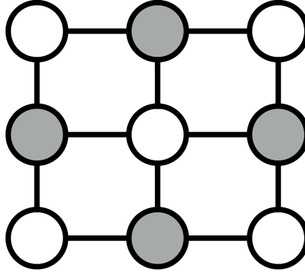
Figure 3.2: The Markov blanket of a node in an Ising model consists of the node’s nearest neighbors (nodes in the Markov blanket of the central node are shaded). Conditioning on the Markov blanket of a node in a graphical model renders it conditionally independent of the rest of the variables. This enables building efficient variational approximations.
