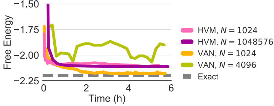
Figure 3.3: Hierarchical variational models (HVMs) scale to statistical physics models with millions of random variables, with over 100x parameter savings. The free energy is reported (the variational lower bound yields an upper bound on the free energy). The HVM variational approximations use 5400 parameters, while the VAN method uses over 700k.
