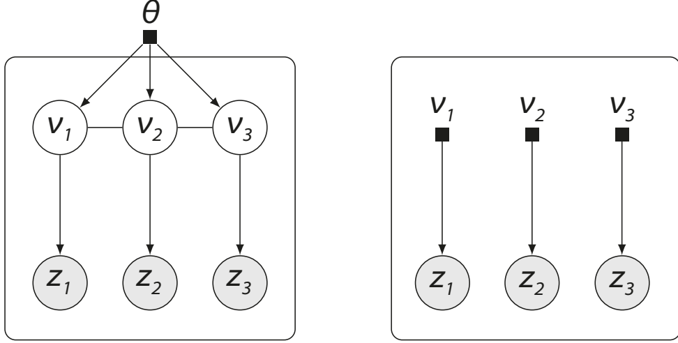
Figure 3.1: Hierarchical variational models (HVMs, left) capture dependencies between latent variables, compared to the mean field variational family with independent variables (right).
