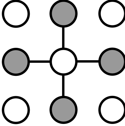
Figure 2.4: The structure of an Ising model can inform variational approximations. This graphical model illustrates a Markov blanket in the Ising model of Figure 2.1 . The Markov blanket of a node is the set of nodes whose values need to be fixed to render a node independent of the rest of the graph. In an Ising model, only neighboring random variables interact and therefore comprise the Markov blanket of a node. Here, the Markov blanket of the central node are shaded, indicating that their values are fixed. The missing edges between the peripheral nodes indicate that the central node is independent of the rest of the graph, conditional on its Markov blanket.
