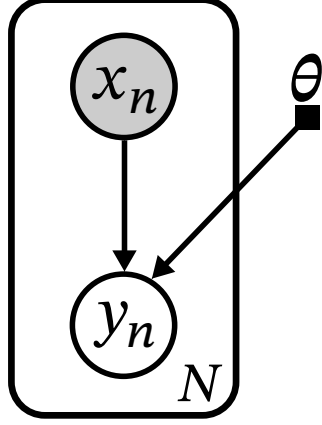
Figure 2.2: Binary classification is a probabilistic modeling technique used in recommender systems. Observed random variables are denoted by shaded nodes, and directed edges in the graph indicated conditional dependence on a node’s parents. There are N independent, identically distributed observations (y_n, x_n) ; the rectangular plate denotes repetition of nodes and edges. The model predicts a binary response y_n using parameters \theta and covariates x_n .
