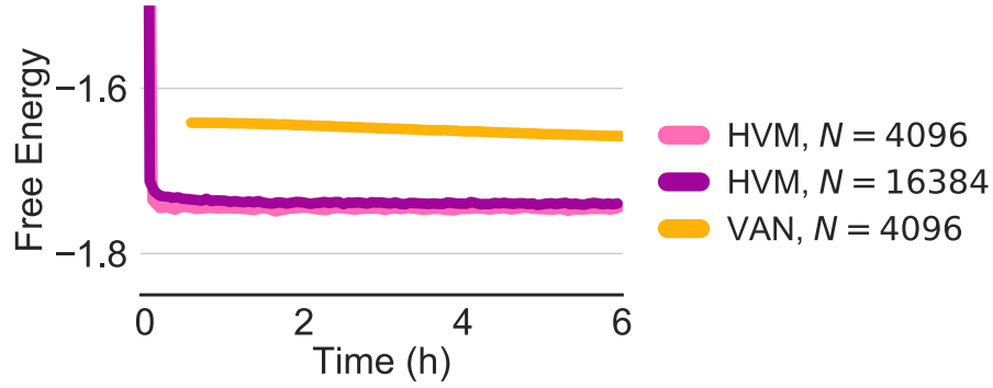
Figure 3.5: Hierarchical variational models (HVMs) scale to larger systems than variational autoregressive network (VAN) models (Wu et al., 2019) when fit to the Sherrington-Kirkpatrick model using variational inference. (Lower is better, as the variational lower bound yields an upper bound on the free energy.) For the system with N = 4096 variables the VAN method completed fewer than ten iterations, and with N = 16384 did not complete a single iteration.
