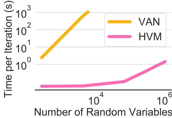
Figure 3.4: Hierarchical variational models (HVMs) are faster than Variational autoregressive networks (VANS) (Wu et al., 2019) and scale to larger systems. The scaling of both variational approximations is illustrated with the time taken per iteration in Ising models. The HVM variational approximations use 5400 parameters and the VAN method uses over 700k. The VAN approximation runs out of memory with 16384 random variables, while the HVM method scales to models with over 1M random variables.
