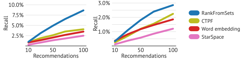
(a) Recall for in-matrix (left) and out-matrix (right) documents.
