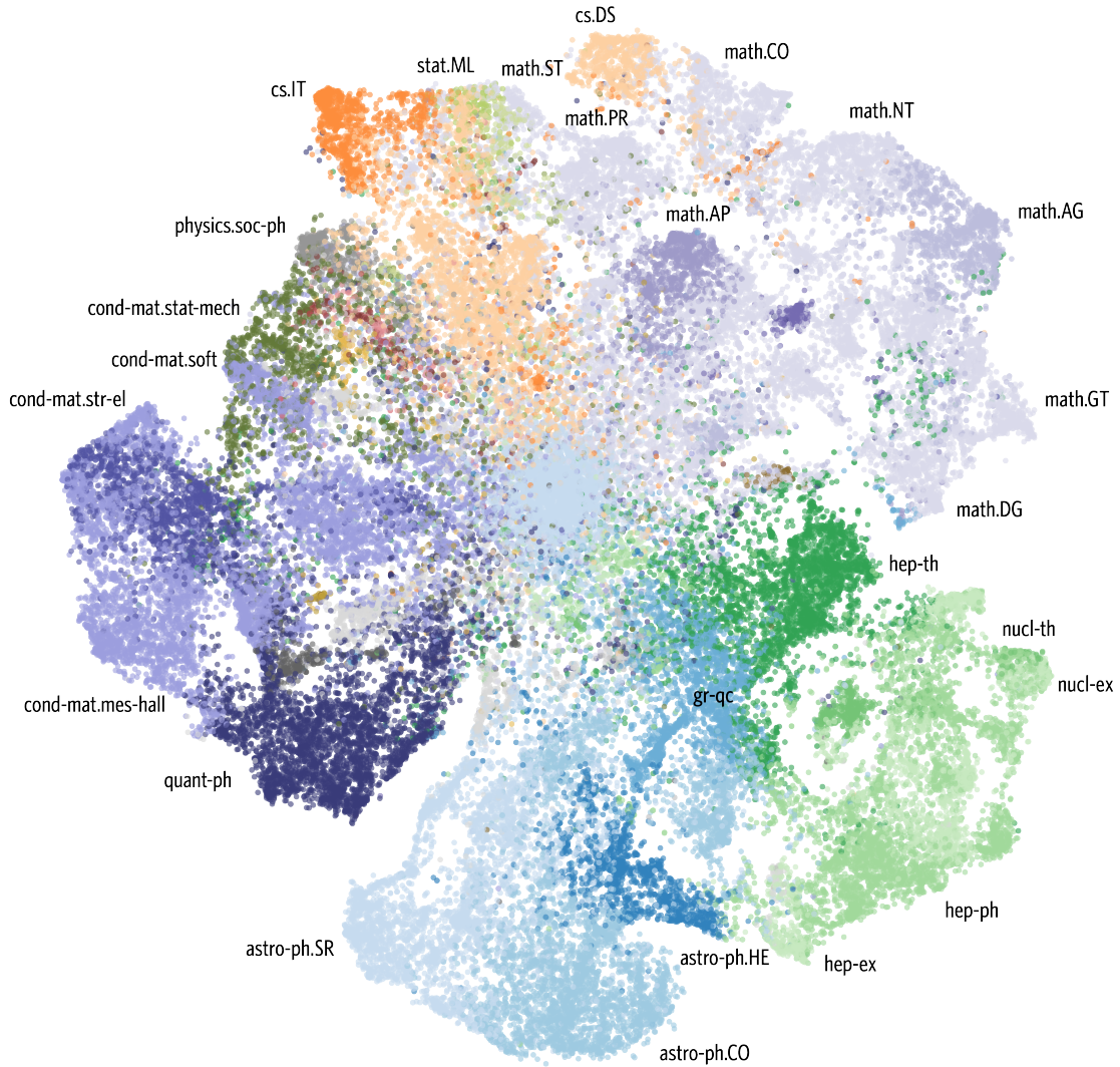
Figure 4.1: RANKFROMSETS trained on arXiv reading behavior clusters researchers by their most frequently-read arXiv category (best viewed on a screen). RFS is trained to recommend items using their attributes (words in the abstract). t-SNE (Maaten and Hinton, 2008) is used to visualize the user embeddings \theta_u in the inner product regression function in Equation (4.2). Each marker represents a user embedding; its color represents a user's most-read arXiv category. Unique colors are determined using the most-read categories across the arXiv, and colors are assigned according to the arXiv ontology. RFS captures usage patterns, as fields of study are related by patterns of reading behavior across neighboring fields (e.g. stat.ML and cs.IT).
