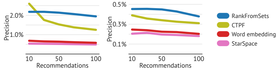
(b) Precision for in-matrix (left) and out-matrix (right) documents.
