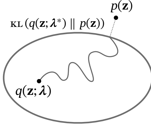
Figure 2.3: Variational inference finds the member of the variational family closest to the target distribution. The oval in the cartoon represents the space of variational approximations q(\mathbf{z}; \lambda) , and the goal of variational inference is to find variational parameters \lambda^* that yield an approximation close to the target probability model p(\mathbf{z}) . One way to measure the distance between a variational approximation and the target probability distribution is with the Kullback-Leibler (KL) divergence.
