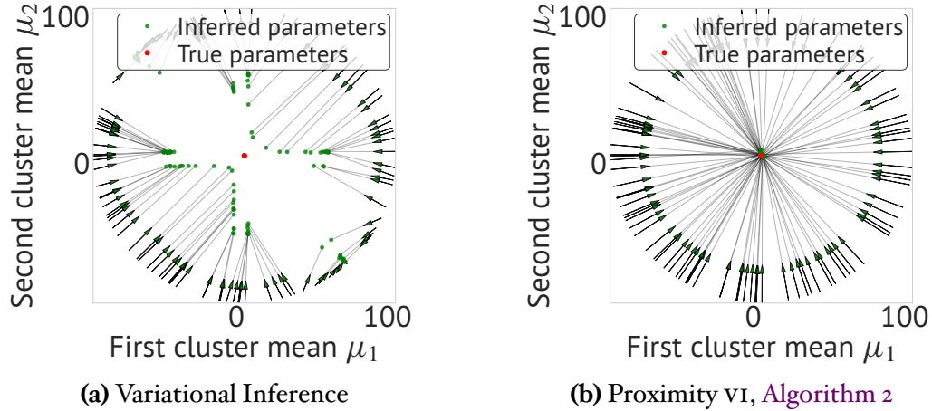
Figure 5.1: Proximity variational inference is robust to bad initialization. We study a Bernoulli factor model. Model parameters are randomly initialized on a ring around the known true parameters (in red) used to generate the data. The arrows start at these parameter initializations and end at the final parameter estimates (shown as green dots). (a) Variational inference with gradient ascent suffers from multiple local optima and cannot reliably recover the truth. (b) PVI with an entropy proximity statistic reliably infers the true parameters using Algorithm 2.
