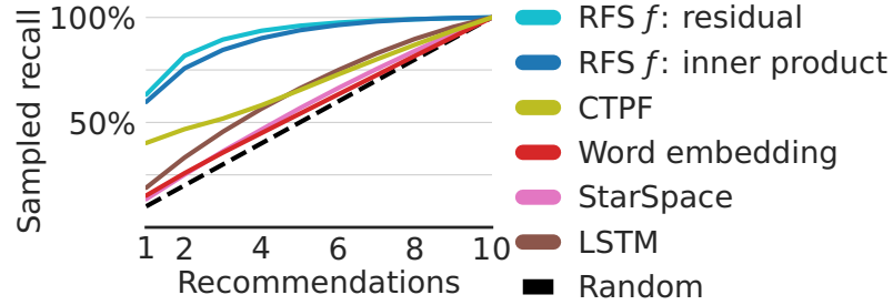
Figure 4.3: RANKFROMSETS models outperform competitors in meal recommendation in terms of sampled recall computed using Equation (4.6). Comparison models are described in Section 4.3 (see Section 4.7.1 for hyperparameters). The RFS regression functions f are defined in Equations (4.2) to (4.4) for the inner product, neural network, and residual models, respectively.
